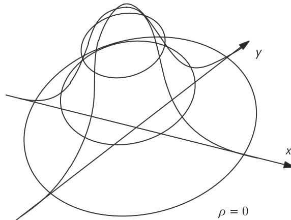
Figure 3.7 Density of a bivariate normal distribution with no correlation; that is, \rho = 0 .
