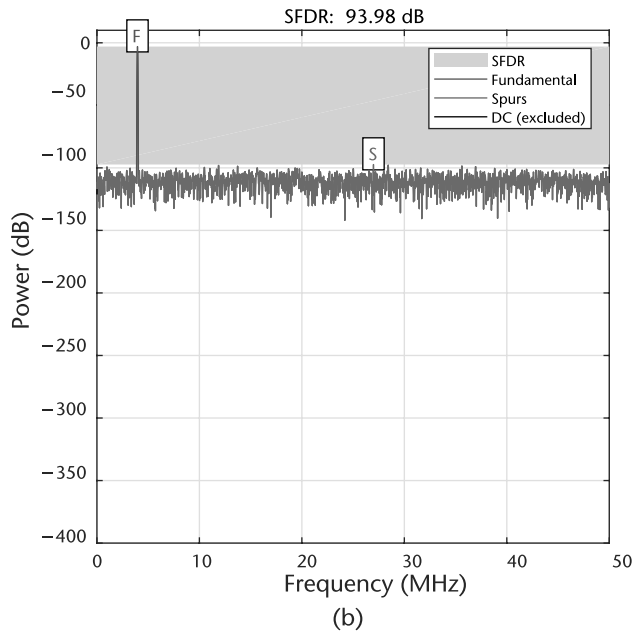
Figure 2.30 SFDR for 12-bit, scaled number. (a) SFDR of fullscale 12-bit fixed point, 1k points, F_A of 3,959,297 Hz, and (b) SFDR of full scale 12-bit fixed point, 10k points, F_A of 3,959,297 Hz.
